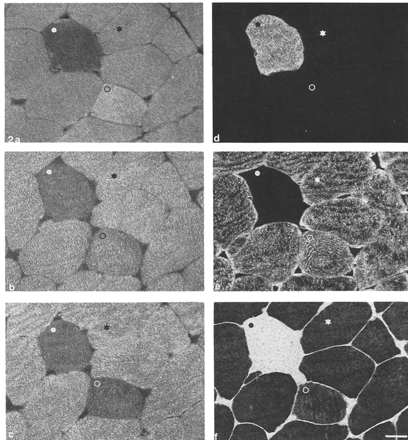
Figure 2. Distribution of the 52,000- and the 170,000-D subunit of the 1,4-dihydropyridine receptor in type I (slow) and type II (fast) myofibers of rabbit gracilis muscle. Serial transverse cryosections of unfixed rabbit gracilis muscle were immunofluorescently labeled with mAb VD 21 (a) to the \beta -subunit of the 1,4-dihydropyridine receptor, with mAb IIC12 (b) and mAb IIID5 (c) to the \alpha_1 -subunit of the 1,4-dihydropyridine receptor, with mAb IID8 (d) and mAb IIH11 (e), respectively specific for the SR-Ca 2+ -ATPase of the type I (slow) and type II (fast) myofibers of rabbit skeletal muscle and histochemically stained for alkali-stable myosin ATPase (f), a marker for type II (fast) myofibers. Note that three classes of fibers can be distinguished after labeling with either mAb VD 21 (a), mAb IIC12 (b), or mAb IIID5 (c). One class is relatively intensely labeled with all three mAbs (a, b, and c, star ); a second class is relatively weakly labeled with all three mAbs (a, b, and c, solid circle ); a third class is more intensely labeled with mAb VD 21 (a; open circle ) but labeled with medium and low intensity by mAb IIC12 (b; solid circle ) and mAb IIID5 (c; solid circle ), respectively. The weakly labeled myofibers (a, b, and c, solid circle ) correspond to type I (slow) fibers (d, e, and f, solid circle ) while the remaining fibers correspond to type II (fast) fibers (d, e, and f, star and open circle ). Bar, 20 \mu m.
